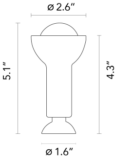
Lamping (Bulb) 5W LED - E12 Candelabra base - 350 Lumens
