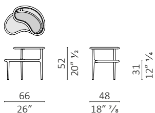
Fagiolo DX/RH piano in vetro e marmo / glass and marble top
