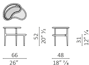
Fagiolo SX/LH piano in vetro e marmo / glass and marble top
