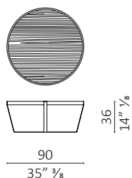
DC occasional table top ottone brunito / burnished brass top
