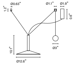
Milana 32 Counterweight
