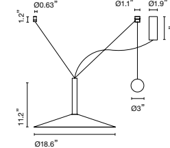
Milana 47 Counterweight
