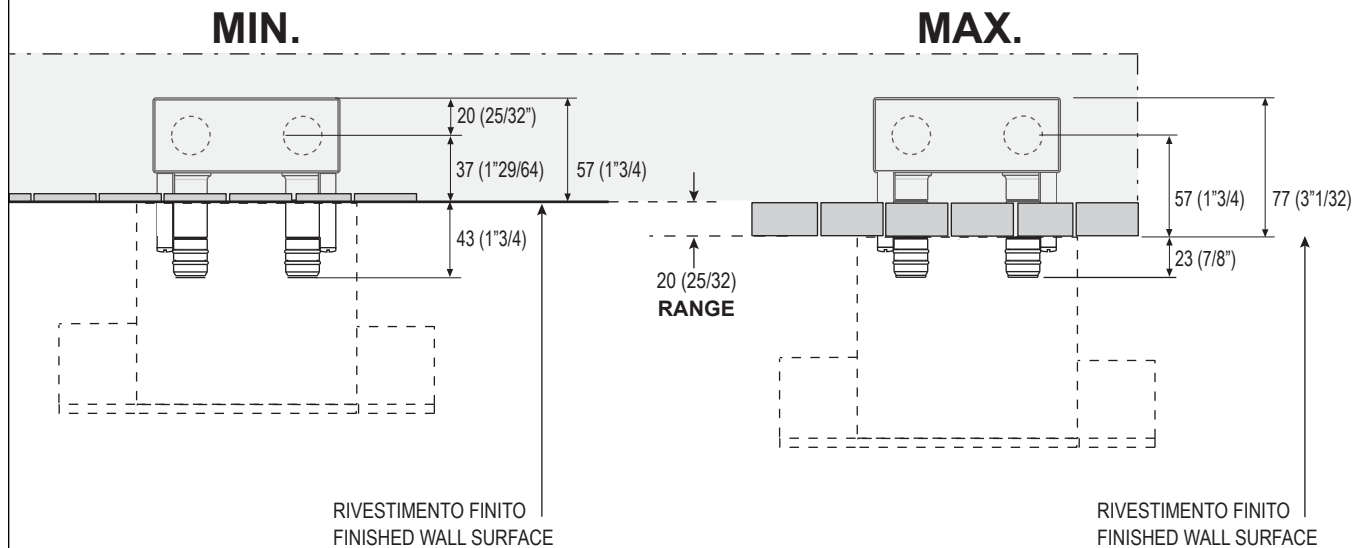
Pianta / Plan view
