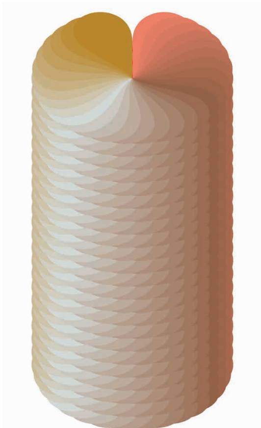
STANDARD MODEL
