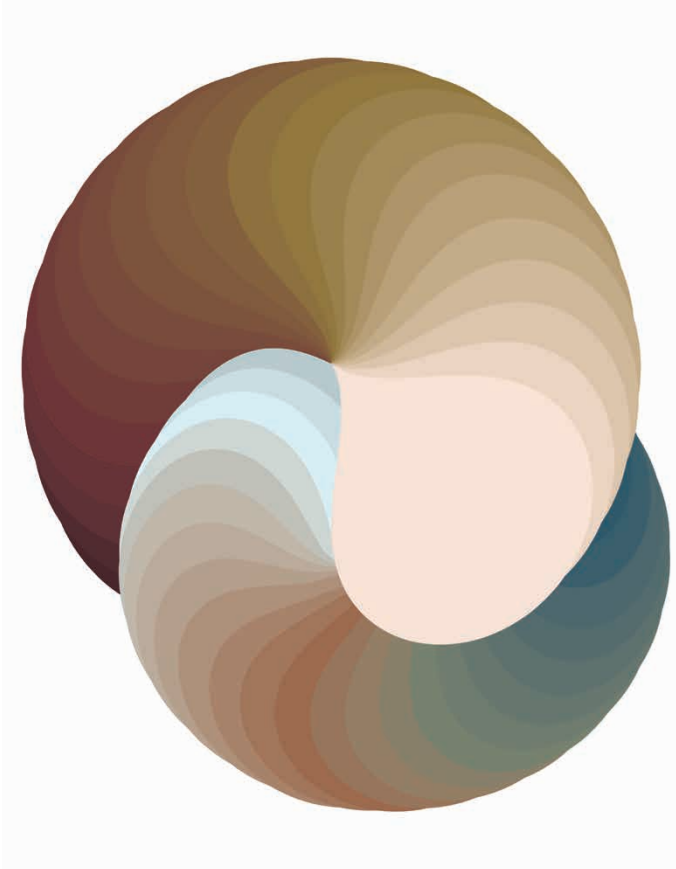
STANDARD MODEL
